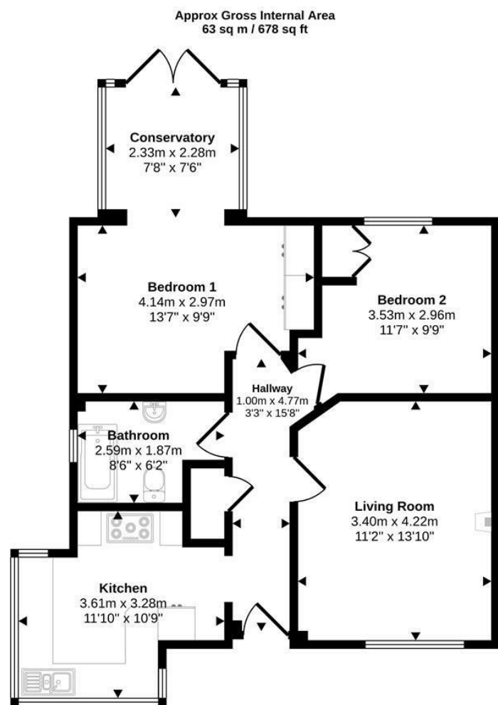
Floorplan
